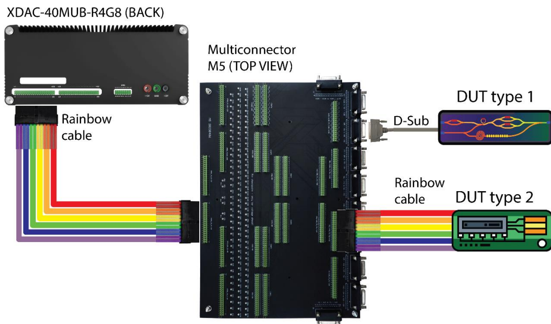
Figure 3. Multi-connectors testing configuration
